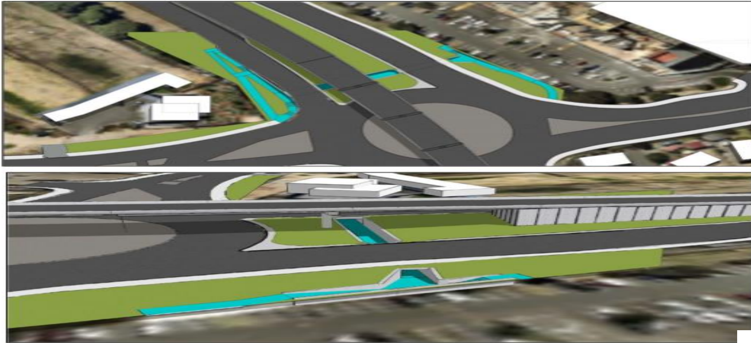
Option 5: Extend existing underpass and provide a new SH2 bridge span
